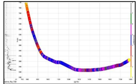
LateralScience trajectory plot on subject well
