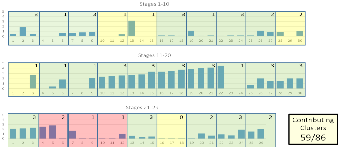
Production log flow profile on subject well
